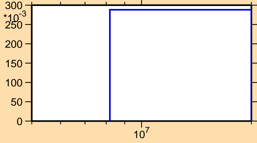
\sigma vs. E for ^{97}\text{Rh}(n,2n)
