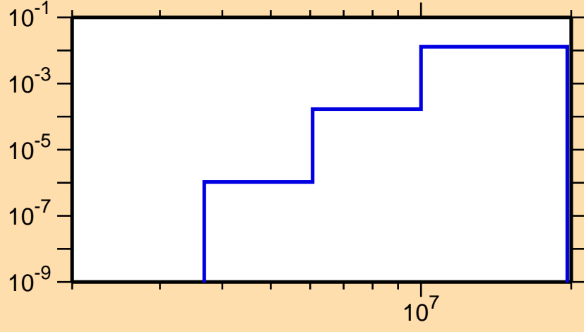
\sigma vs. E for ^{98}\text{Rh}(n,d)
