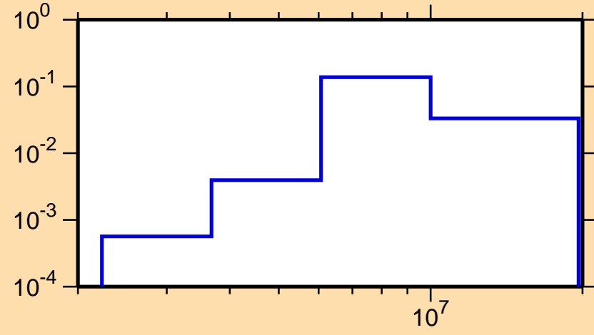
\sigma vs. E for ^{98}\text{Rh}(n,n\text{cont.})
