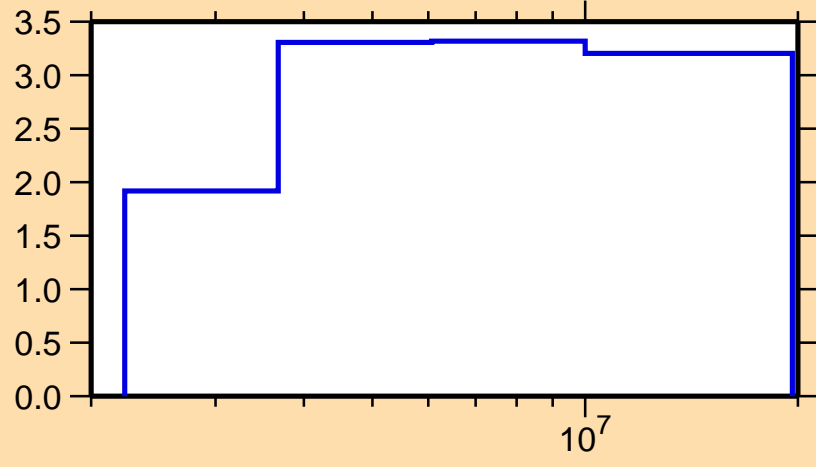
\Delta\sigma/\sigma vs. E for ^{98}\text{Rh}(n,n\text{onel.})
