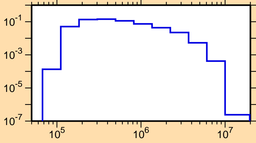
\sigma vs. E for ^{98}\text{Rh}(n,n_1)
