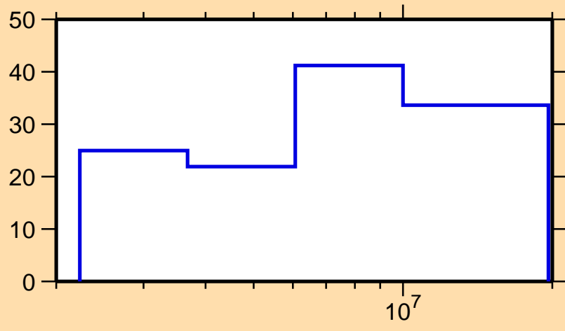
\Delta\sigma/\sigma vs. E for ^{98}\text{Rh}(n,n\text{cont.})
