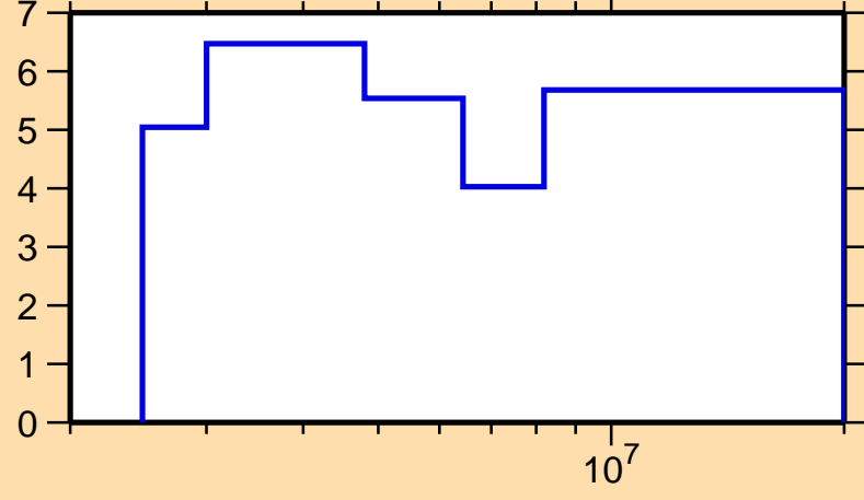
\Delta\sigma/\sigma vs. E for ^{98}\text{Rh}(n,\text{tot.})
