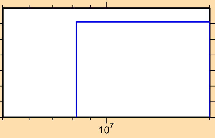
\sigma vs. E for ^{98}\text{Rh}(n,3n)
