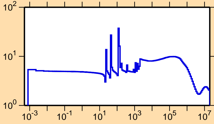
\sigma vs. E for ^{99}\text{Rh}(n,\text{el.})
