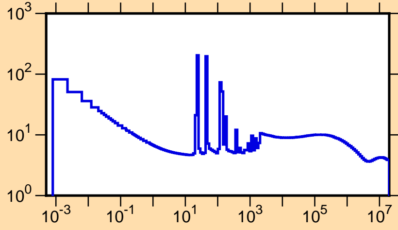
\sigma vs. E for ^{99}\text{Rh}(n,\text{tot.})
