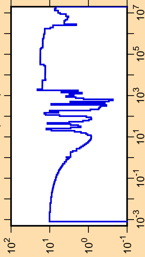
\Delta\sigma/\sigma vs. E for ^{99}\text{Rh}(n,\text{tot.})
