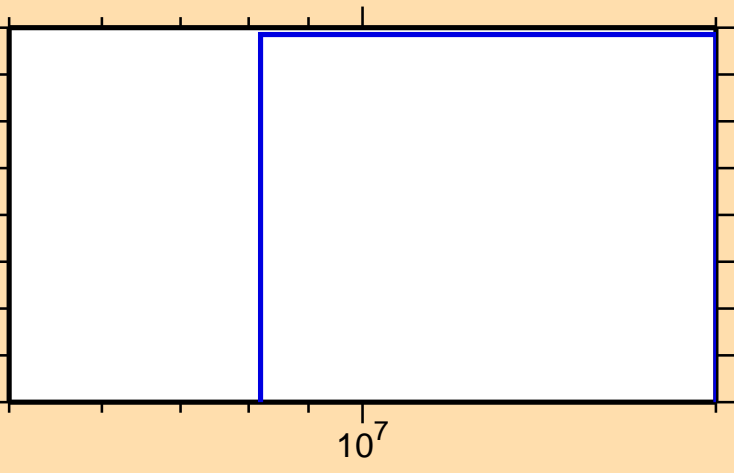
\sigma vs. E for ^{99}\text{Rh}(n,\text{He3})
