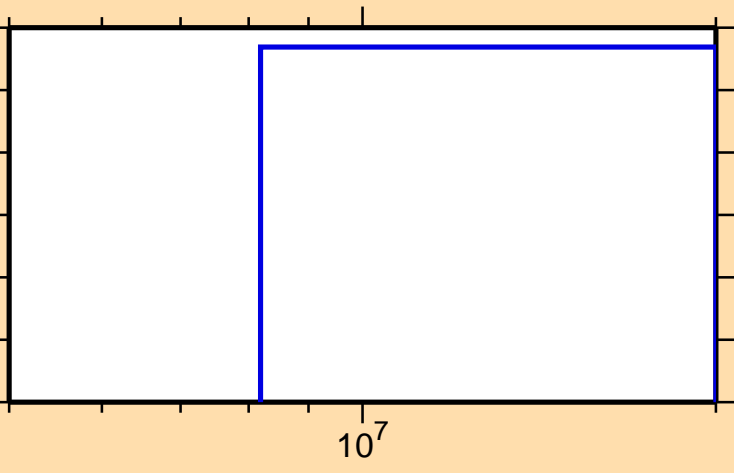
\sigma vs. E for ^{99}\text{Rh}(\text{mt117})
