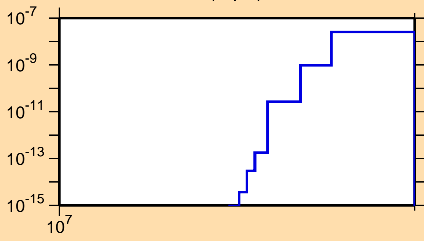
\sigma vs. E for ^{99}\text{Rh}(n,\text{pd})
