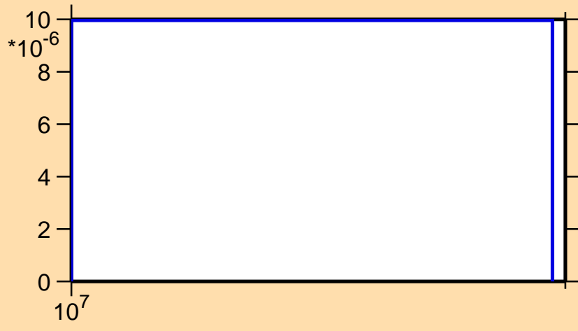
\sigma vs. E for ^{99}\text{Rh}(n,2np)
