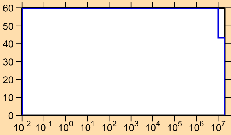
\Delta\sigma/\sigma vs. E for ^{99}\text{Rh}(n,p)
