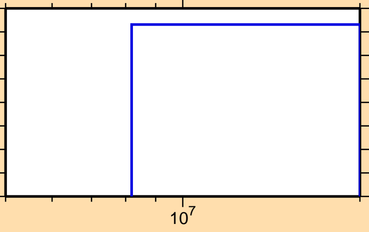
\sigma vs. E for ^{99}\text{Rh}(n,\text{nd})
