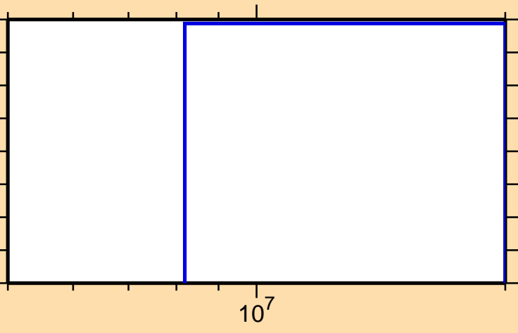
\sigma vs. E for ^{99}\text{Rh}(n,\text{He3})
