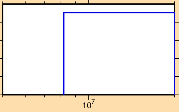
\sigma vs. E for ^{99}\text{Rh}(n,2np)
