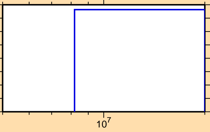
\sigma vs. E for ^{99}\text{Rh}(n,\text{pt})
