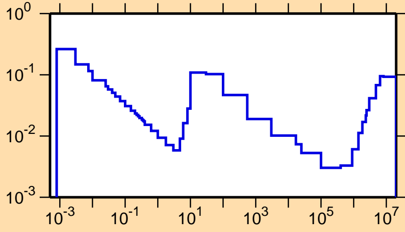
\sigma vs. E for ^{99}\text{Rh}(n,p)
