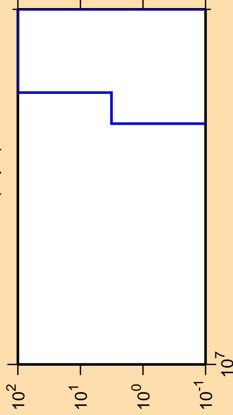
\Delta\sigma/\sigma vs. E for ^{100}\text{Rh}(n,pd)
