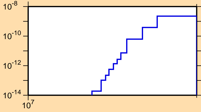
\sigma vs. E for ^{100}\text{Rh}(\text{mt117})
