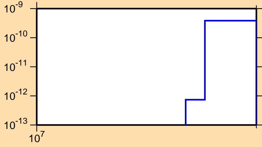
\sigma vs. E for ^{100}\text{Rh}(n,pd)
