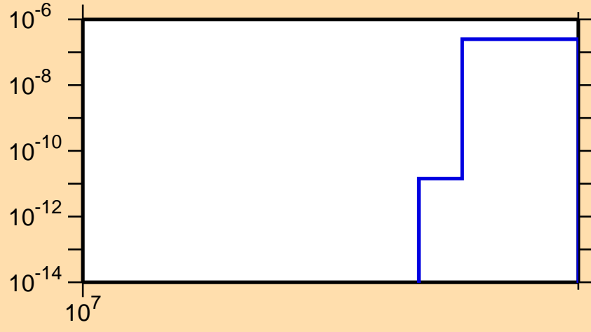
\sigma vs. E for ^{100}\text{Rh}(n,nt)
