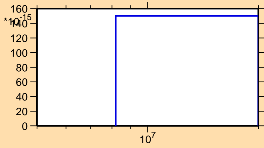
\sigma vs. E for ^{100}\text{Rh} (mt 34)
