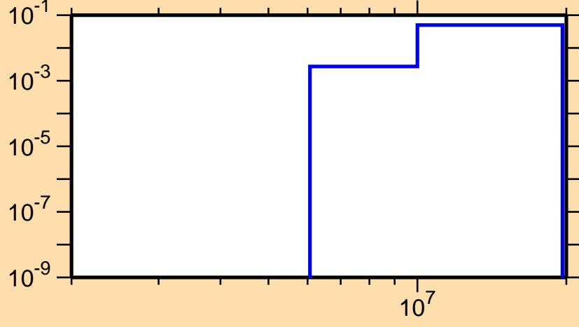
\sigma vs. E for ^{101}\text{Rh}(n,np)
