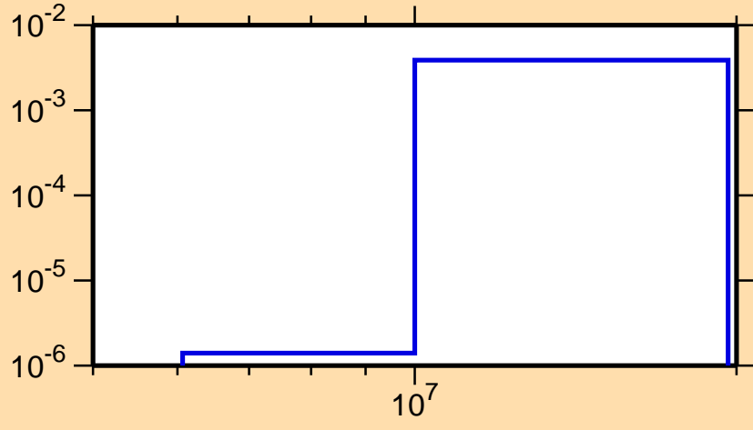
\sigma vs. E for ^{101}\text{Rh}(n,n\alpha)
