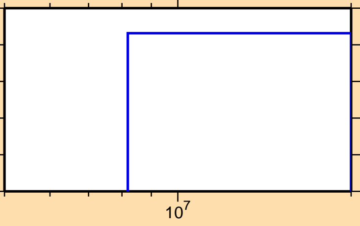
\sigma vs. E for ^{101}\text{Rh}(\text{mt117})
