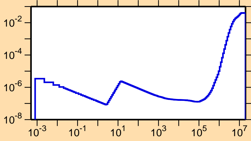
\sigma vs. E for ^{101}\text{Rh}(n,p)
