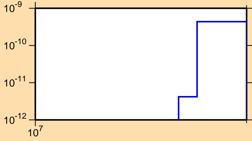
\sigma vs. E for ^{101}\text{Rh} (mt 45)
