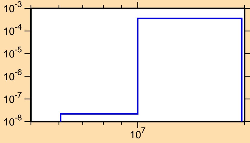
\sigma vs. E for ^{102}\text{Rh}(n,t)
