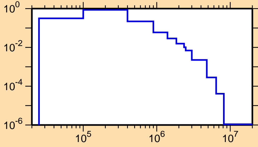
\sigma vs. E for ^{102}\text{Rh}(n,n_1)
