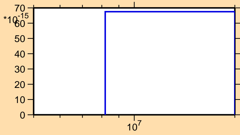
\sigma vs. E for ^{102}\text{Rh}(\text{mt117})
