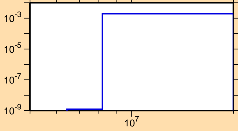
\sigma vs. E for ^{102}\text{Rh}(n,n\alpha)
