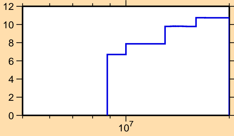
\Delta\sigma/\sigma vs. E for ^{103}\text{Rh}(n,\text{tot.})
