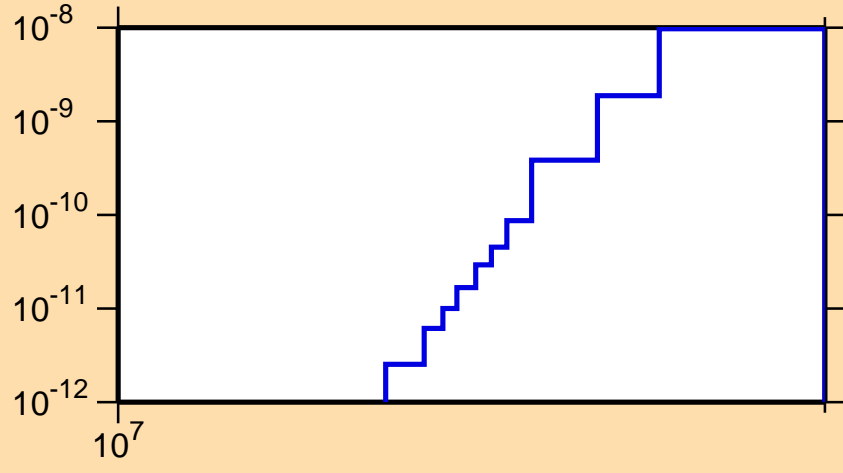
\sigma vs. E for ^{104}\text{Rh}(n,p\alpha)
