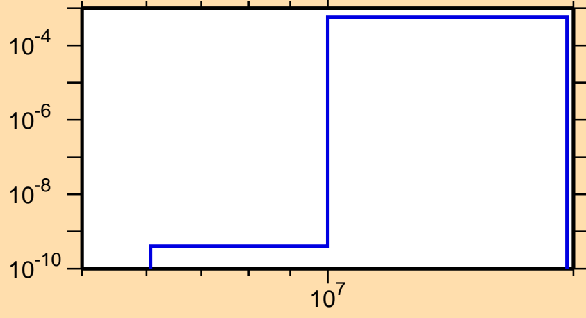
\sigma vs. E for ^{104}\text{Rh}(n,n\alpha)
