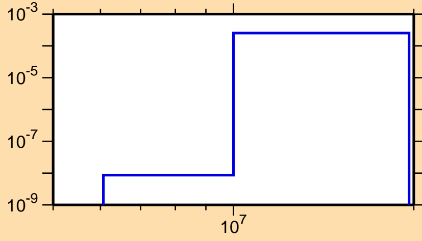
\sigma vs. E for ^{104}\text{Rh}(n,t)
