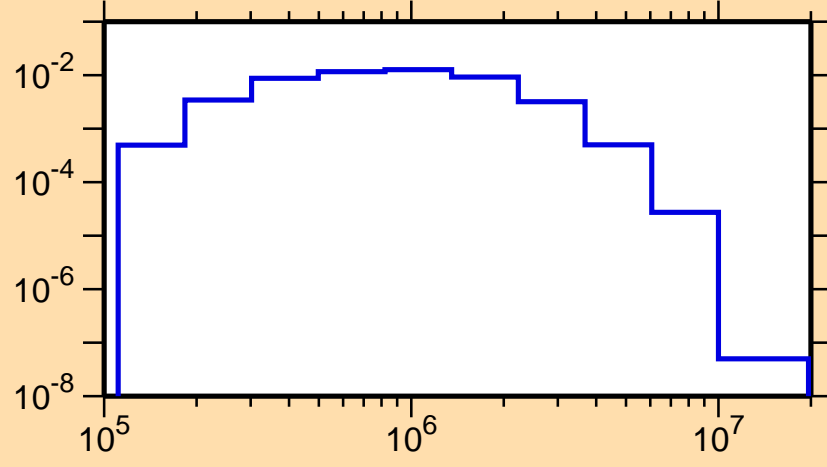
\sigma vs. E for ^{104}\text{Rh}(n,n_3)
