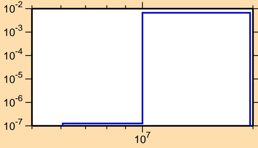
\sigma vs. E for ^{104}\text{Rh}(n,np)
