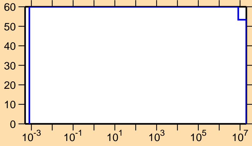
\Delta\sigma/\sigma vs. E for ^{104}\text{Rh}(n,p)
