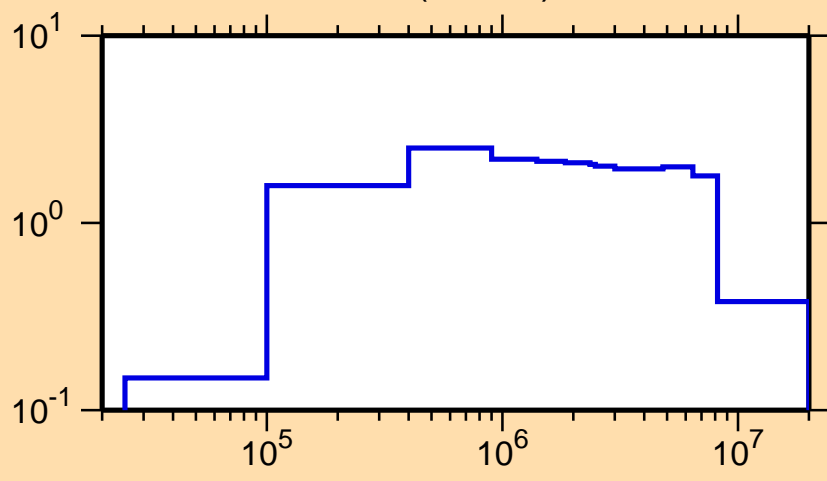
\sigma vs. E for ^{104}\text{Rh}(n,\text{inel.})
