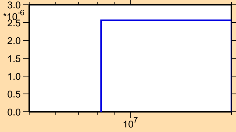
\sigma vs. E for ^{104}\text{Rh}(n,\text{nd})
