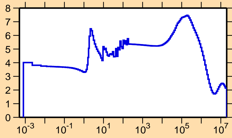
\sigma vs. E for ^{104}\text{Rh}(n,\text{el.})
