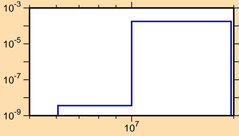
\sigma vs. E for ^{106}\text{Rh}(n,t)
