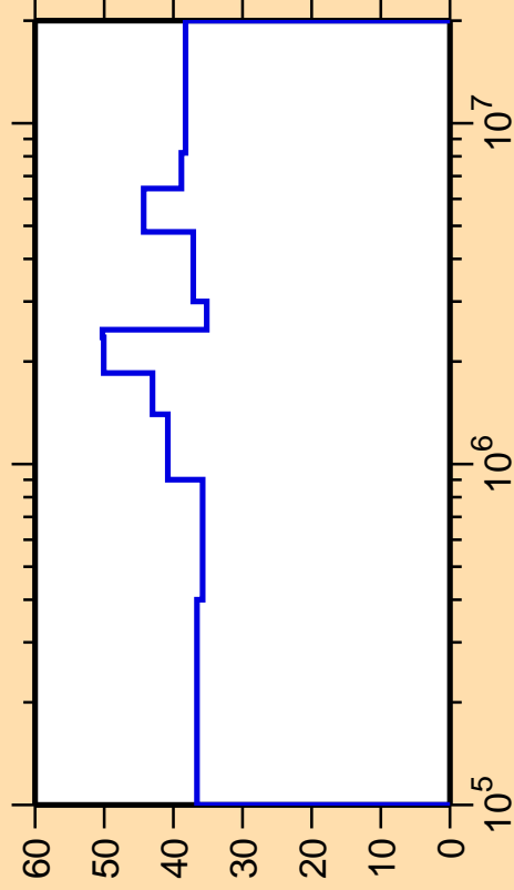
\Delta\sigma/\sigma vs. E for ^{106}\text{Rh}(n,n_1)
