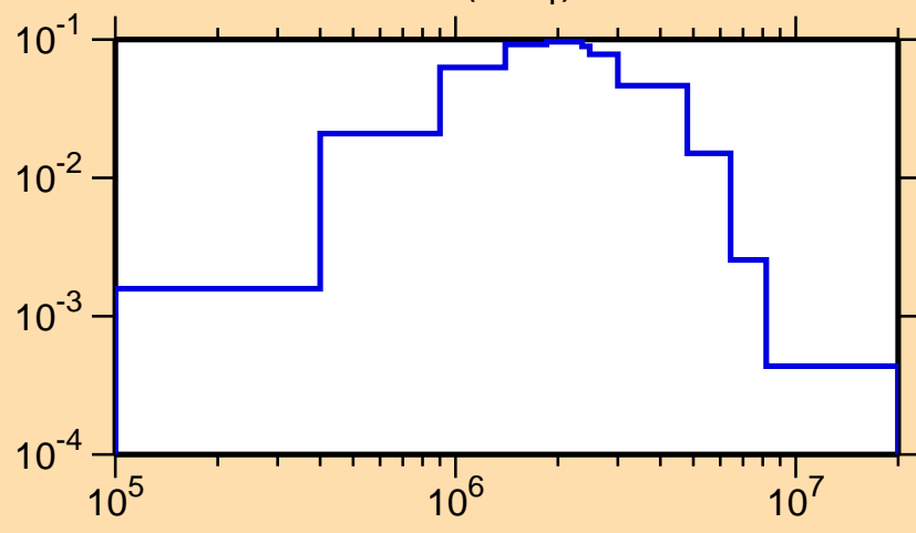
\sigma vs. E for ^{106}\text{Rh}(n,n_1)
