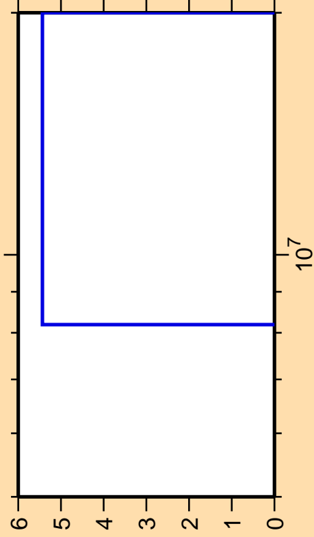
\Delta\sigma/\sigma vs. E for ^{106}\text{Rh}(n,p\alpha)
