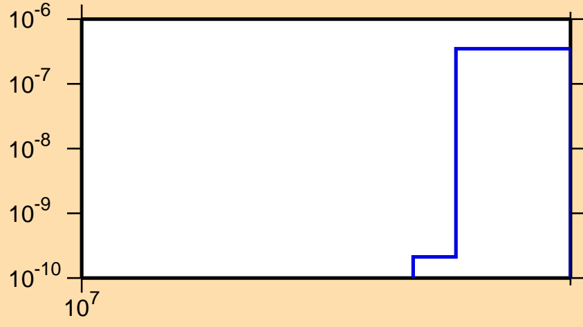
\sigma vs. E for ^{107}\text{Rh}(n,nt)
