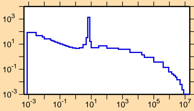
\sigma vs. E for ^{107}\text{Rh}(n,\gamma)
