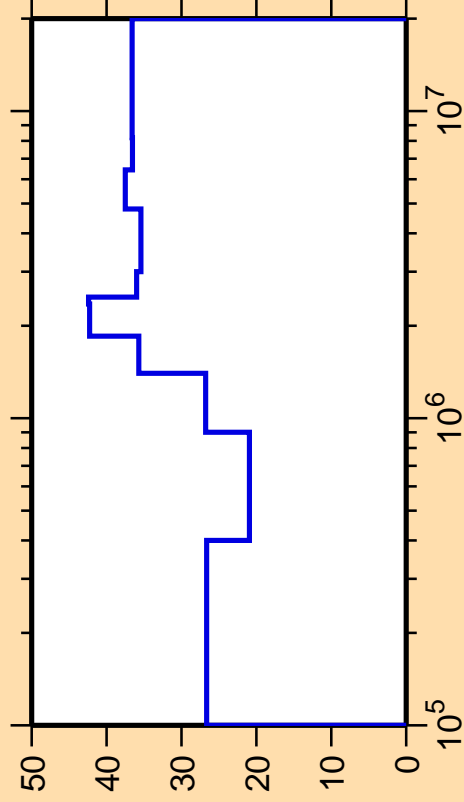
\Delta\sigma/\sigma vs. E for ^{107}\text{Rh}(n,n_1)
