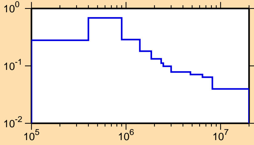
\sigma vs. E for ^{107}\text{Rh}(n,n_1)
