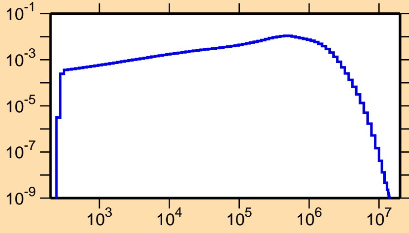
\sigma vs. E for ^{108}\text{Rh}(n,n_1)
