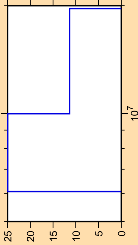
\Delta\sigma/\sigma vs. E for ^{108}\text{Rh}(n,2n)
