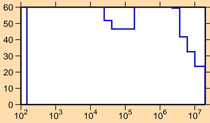
\Delta\sigma/\sigma vs. E for ^{108}\text{Rh}(n,n_1)
