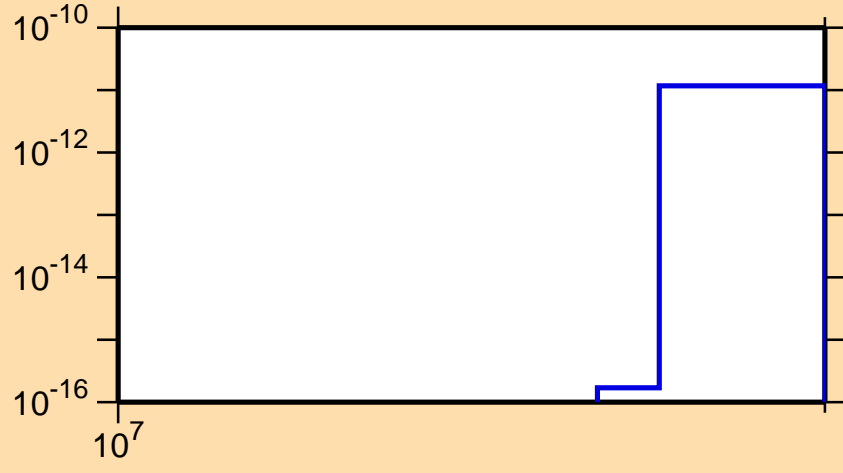
\sigma vs. E for ^{109}\text{Rh}(n,2n\alpha)
