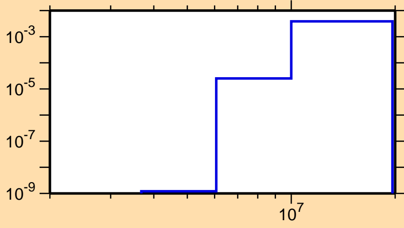
\sigma vs. E for ^{109}\text{Rh}(n,p)
