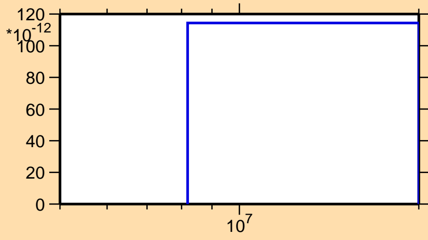
\sigma vs. E for ^{109}\text{Rh}(n,2np)
