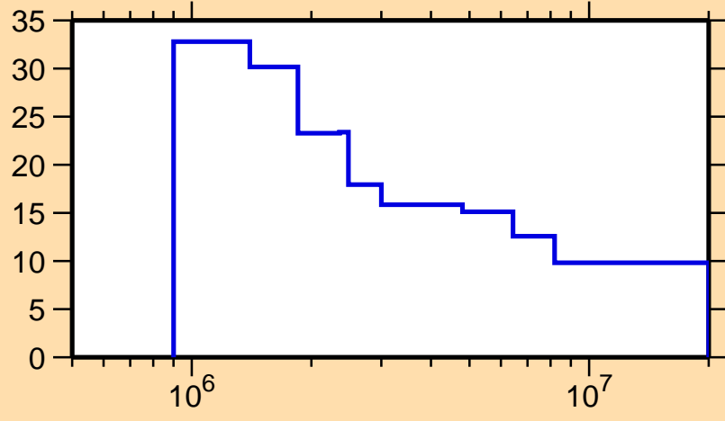
\Delta\sigma/\sigma vs. E for ^{109}\text{Rh}(n,n\text{nonel.})
