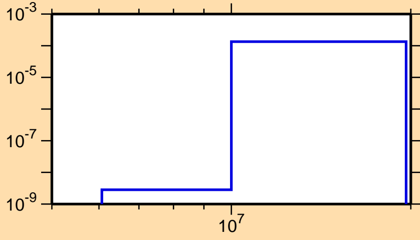
\sigma vs. E for ^{111}\text{Rh}(n,\alpha)
