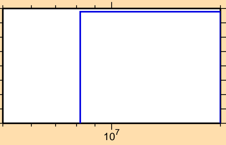
\sigma vs. E for ^{111}\text{Rh}(n,3n)
