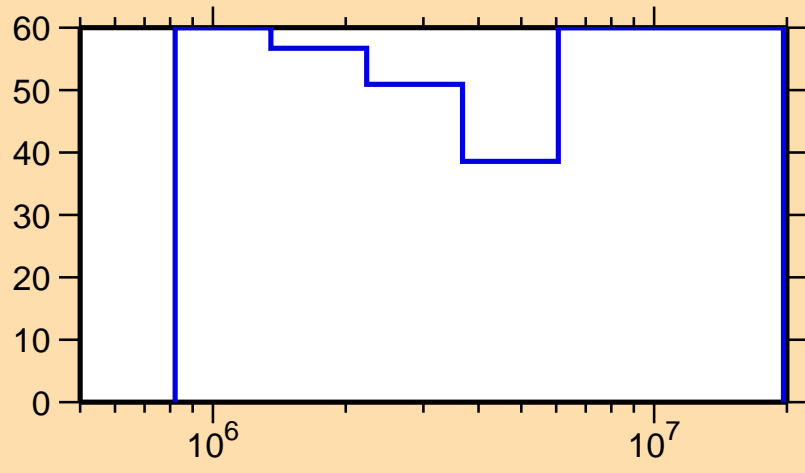
\Delta\sigma/\sigma vs. E for ^{112}\text{Rh}(n,n\text{cont.})
