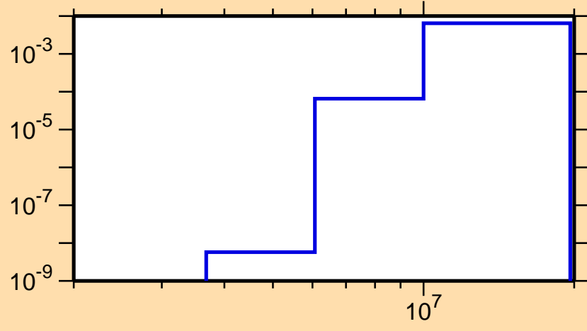
\sigma vs. E for ^{112}\text{Rh}(n,p)
