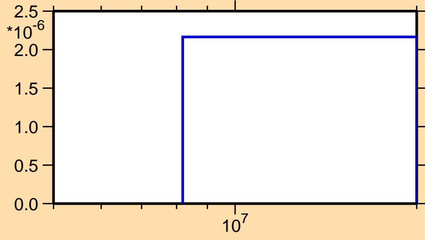
\sigma vs. E for ^{112}\text{Rh}(n,n\alpha)
