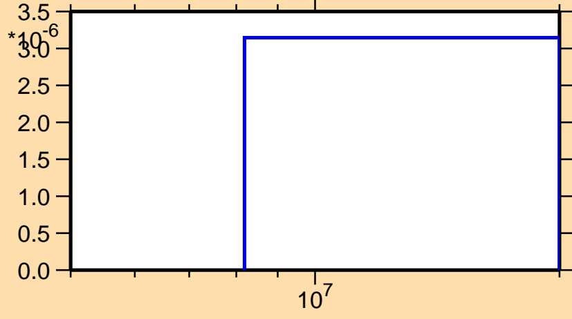
\sigma vs. E for ^{113}\text{Rh}(n,t)
