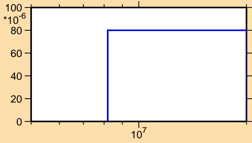
\sigma vs. E for ^{113}\text{Rh}(n,d)
