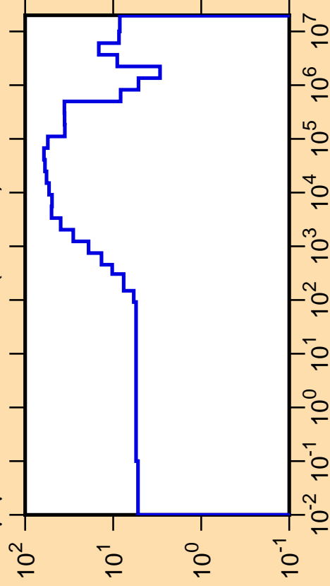
\Delta\mu/\mu vs. E for ^{114}\text{Rh}(\text{mt251})
