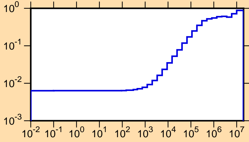
\mu vs. E for ^{114}\text{Rh}(\text{mt251})
