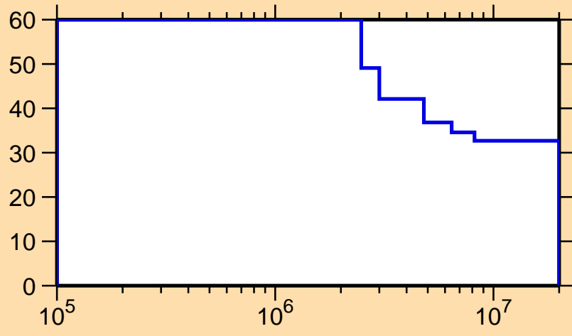
\Delta\sigma/\sigma vs. E for ^{114}\text{Rh}(n,n_1)
