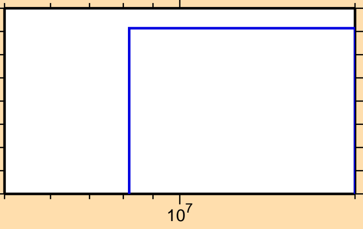
\sigma vs. E for ^{114}\text{Rh}(n,t)
