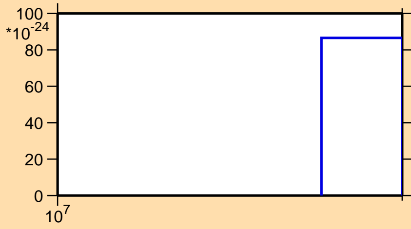
\sigma vs. E for ^{201}\text{Rn}(\text{mt } 11)
