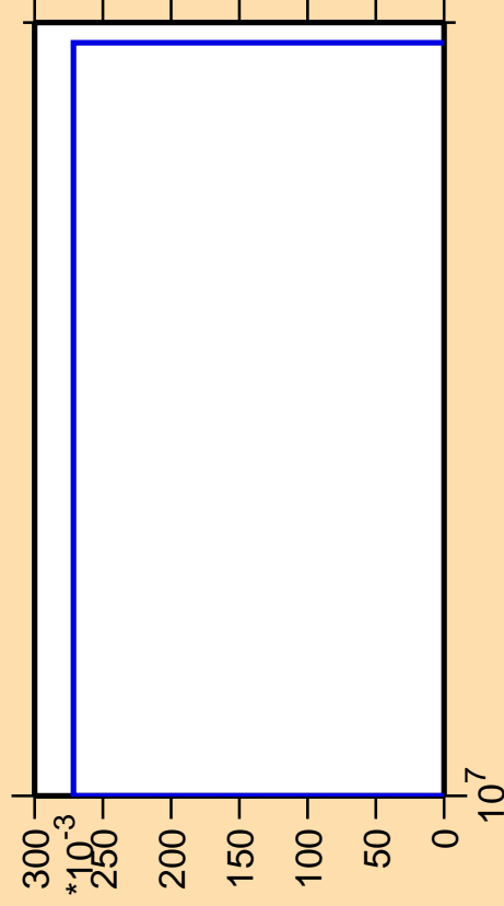
\Delta\sigma/\sigma vs. E for ^{201}\text{Rn}(n,3n\alpha)
