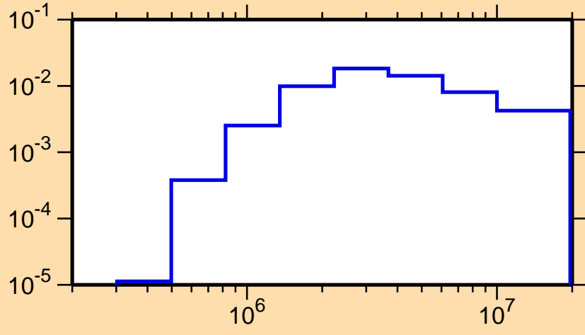
\sigma vs. E for ^{201}\text{Rn}(n,n_3)
