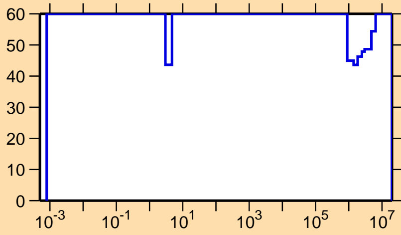
\Delta\sigma/\sigma vs. E for ^{201}\text{Rn}(n,\gamma)
