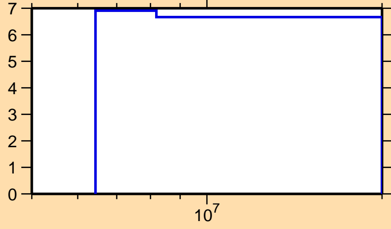
\Delta\sigma/\sigma vs. E for ^{201}\text{Rn}(n,\text{tot.})
