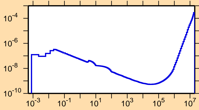
\sigma vs. E for ^{201}\text{Rn}(n,p\alpha)
