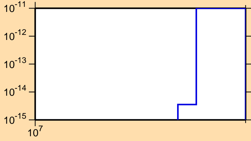
\sigma vs. E for ^{201}\text{Rn}(n,nt)
