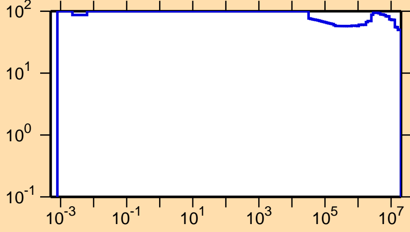
\Delta\sigma/\sigma vs. E for ^{201}\text{Rn}(n,p)
