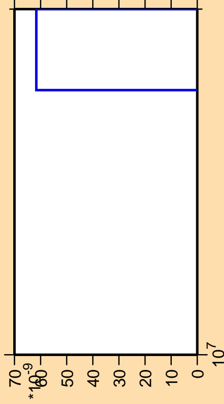
\Delta\sigma/\sigma vs. E for ^{201}\text{Rn}(\text{mt 11})
