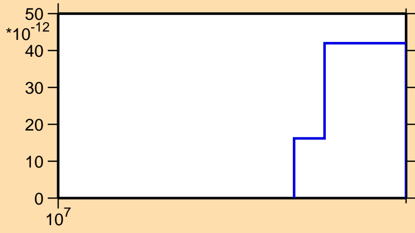
\sigma vs. E for ^{201}\text{Rn}(n,3n\alpha)
