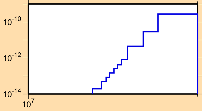
\sigma vs. E for ^{201}\text{Rn}(\text{mt } 34)
