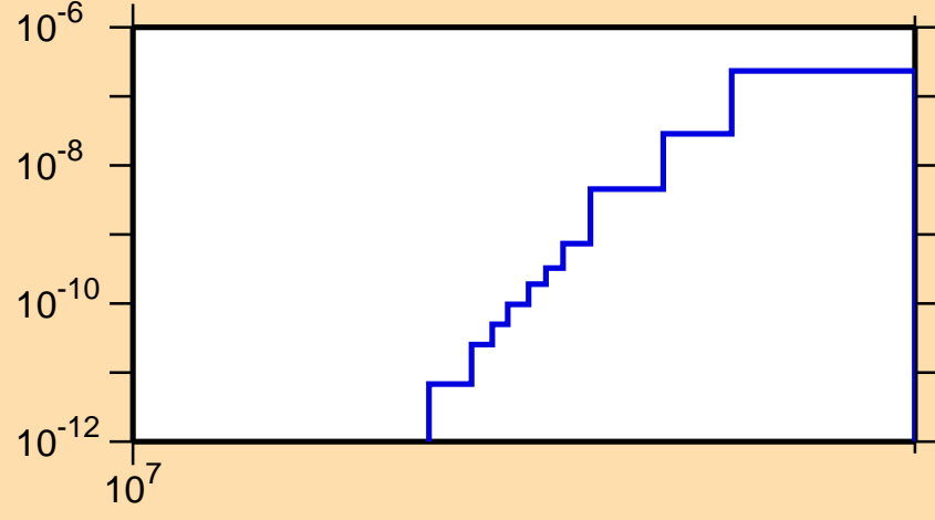
\sigma vs. E for ^{201}\text{Rn}(n,nd)
