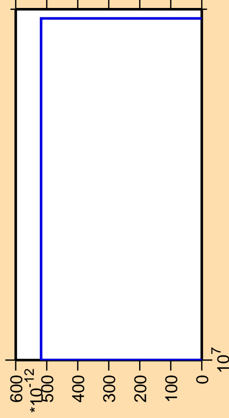
\Delta\sigma/\sigma vs. E for ^{201}\text{Rn} (mt 11)
