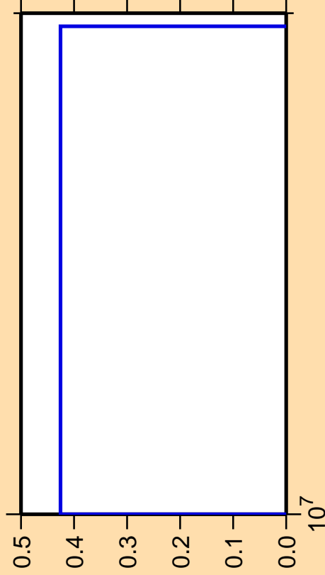
\Delta\sigma/\sigma vs. E for ^{201}\text{Rn}(n,nt)
