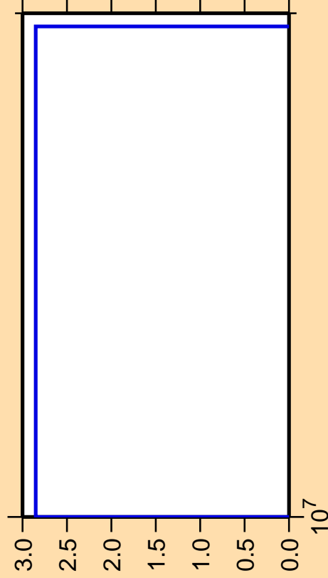
\Delta\sigma/\sigma vs. E for ^{201}\text{Rn}(n,3n\alpha)
