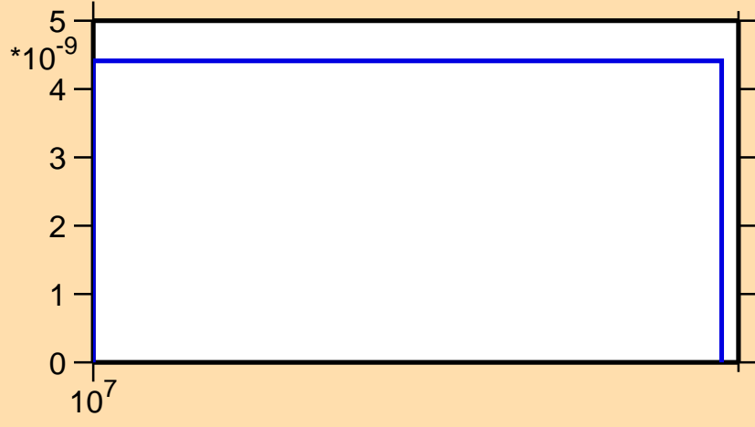
\sigma vs. E for ^{201}\text{Rn}(n,nd)
