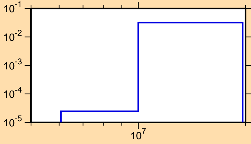
\sigma vs. E for ^{201}\text{Rn}(n,2n)
