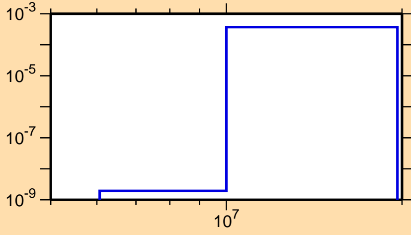
\sigma vs. E for ^{201}\text{Rn}(n,t)
