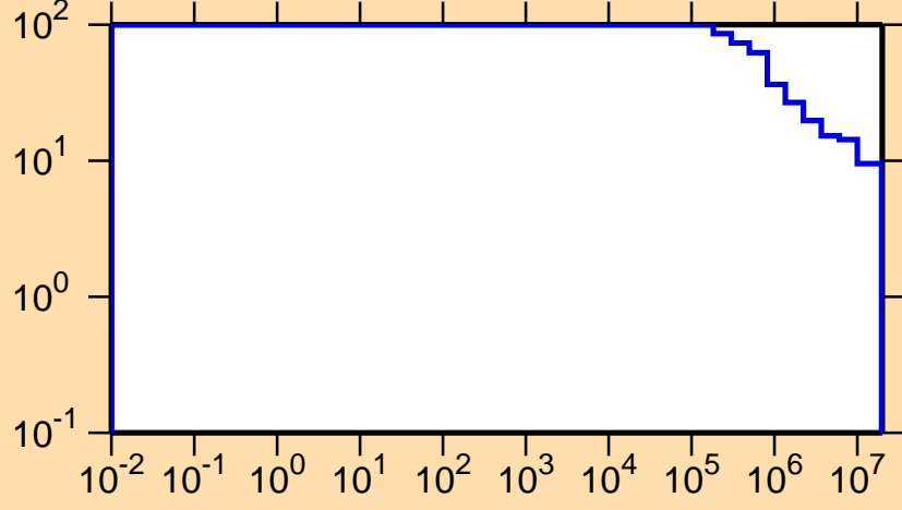
\Delta\sigma/\sigma vs. E for ^{201}\text{Rn}(n,\text{nonel.})
