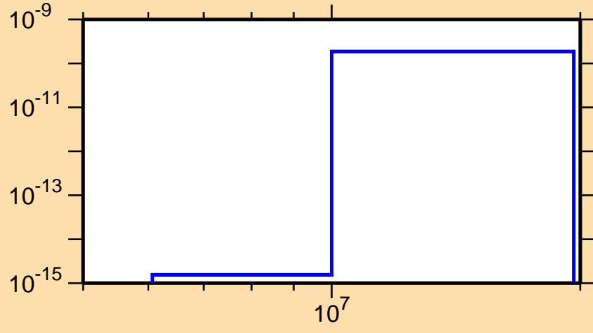
\sigma vs. E for ^{201}\text{Rn}(\text{mt117})
