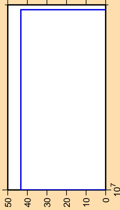
\Delta\sigma/\sigma vs. E for ^{201}\text{Rn} (mt 34)
