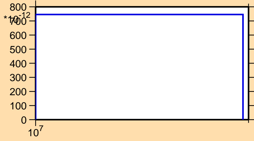
\sigma vs. E for ^{201}\text{Rn}(n,3n)
