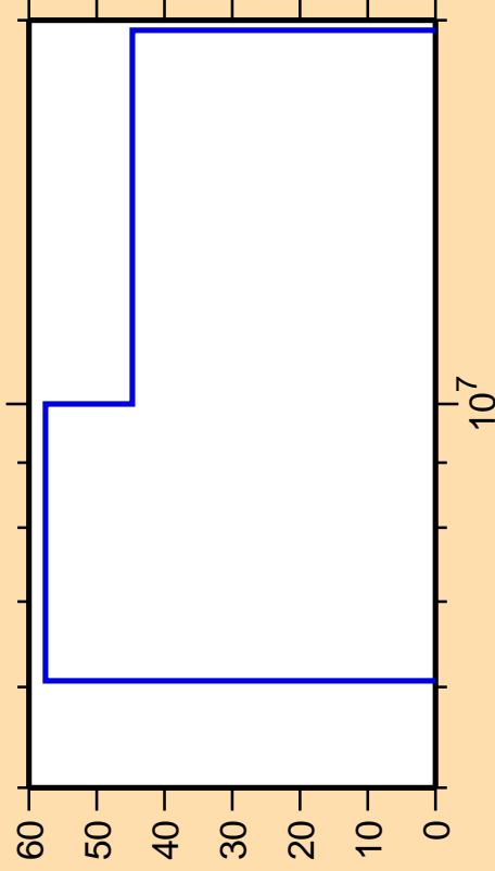
\Delta\sigma/\sigma vs. E for ^{201}\text{Rn}(n,n\text{cont.})
