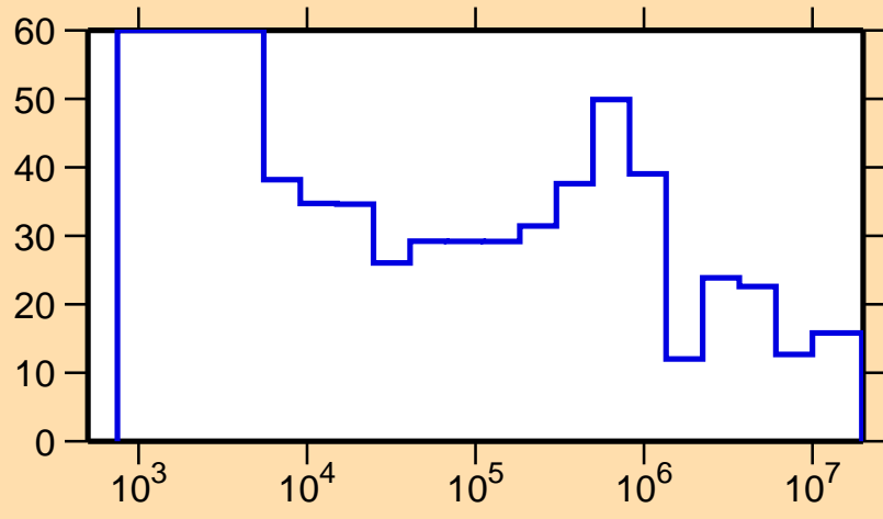
\Delta\sigma/\sigma vs. E for ^{201}\text{Rn}(n,\text{tot.})
