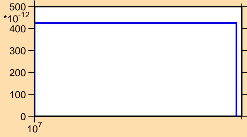
\sigma vs. E for ^{201}\text{Rn}(n,\text{pt})
