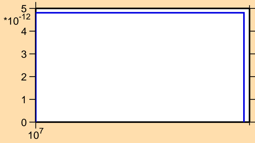
\sigma vs. E for ^{201}\text{Rn} (mt 34)
