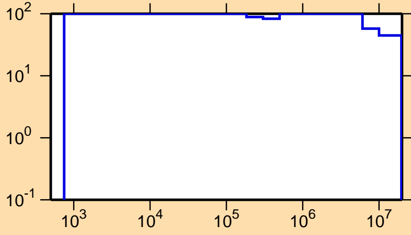
\Delta\sigma/\sigma vs. E for ^{201}\text{Rn}(n,n\text{cont.})
