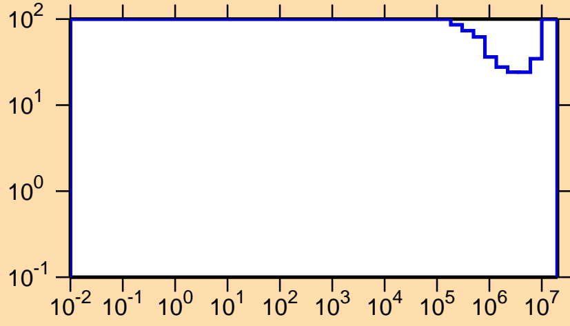
\Delta\sigma/\sigma vs. E for ^{201}\text{Rn}(n,\gamma)
