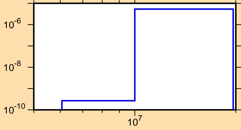
\sigma vs. E for ^{201}\text{Rn}(n,\text{He3})
