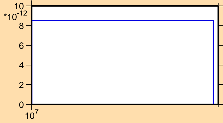
\sigma vs. E for ^{201}\text{Rn}(n,3n\alpha)
