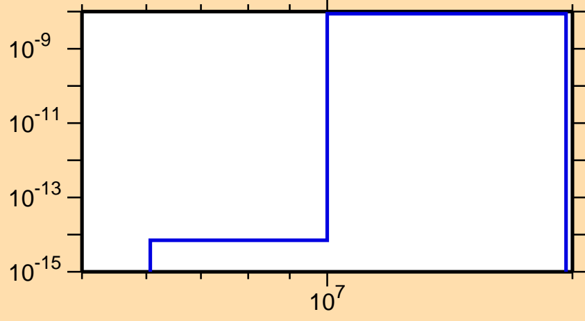
\sigma vs. E for ^{201}\text{Rn}(\text{mt } 45)
