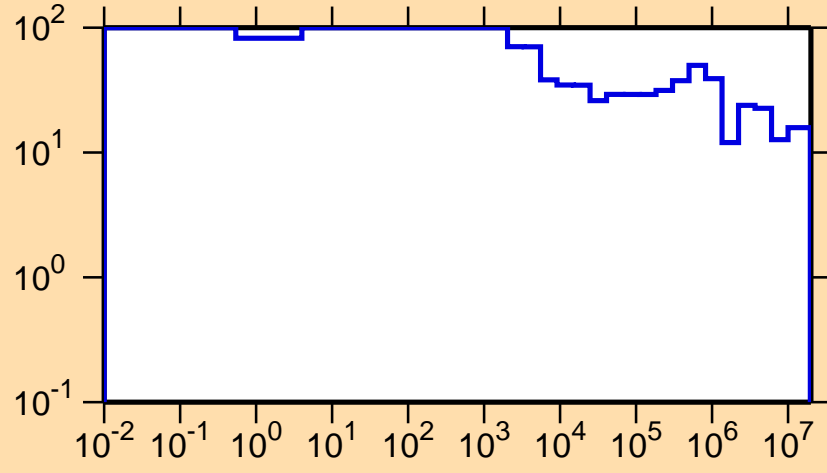
\Delta\sigma/\sigma vs. E for ^{201}\text{Rn}(n,\text{tot.})
