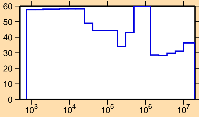
\Delta\sigma/\sigma vs. E for ^{201}\text{Rn}(n, \text{el.})
