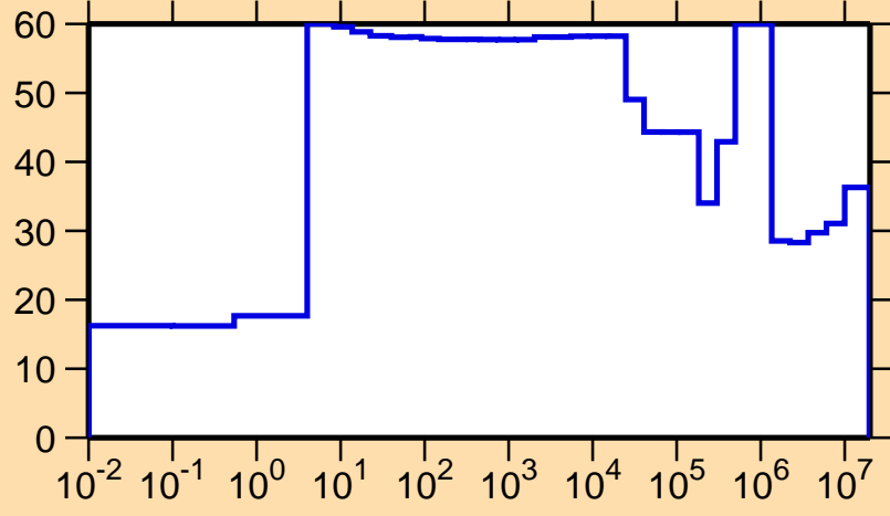
\Delta\sigma/\sigma vs. E for ^{201}\text{Rn}(n,\text{el.})
