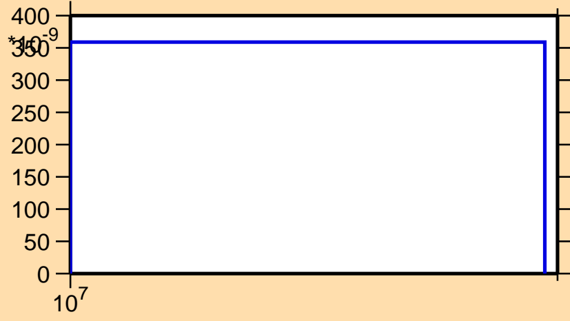
\sigma vs. E for ^{201}\text{Rn}(n,2np)
