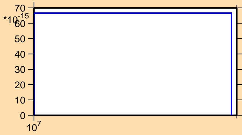
\sigma vs. E for ^{201}\text{Rn}(n,nt)
