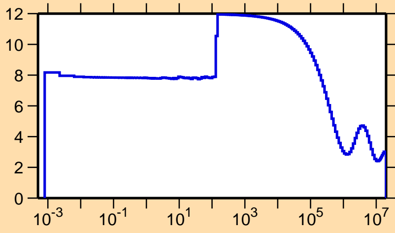
\sigma vs. E for ^{202}\text{Rn}(n,\text{el.})
