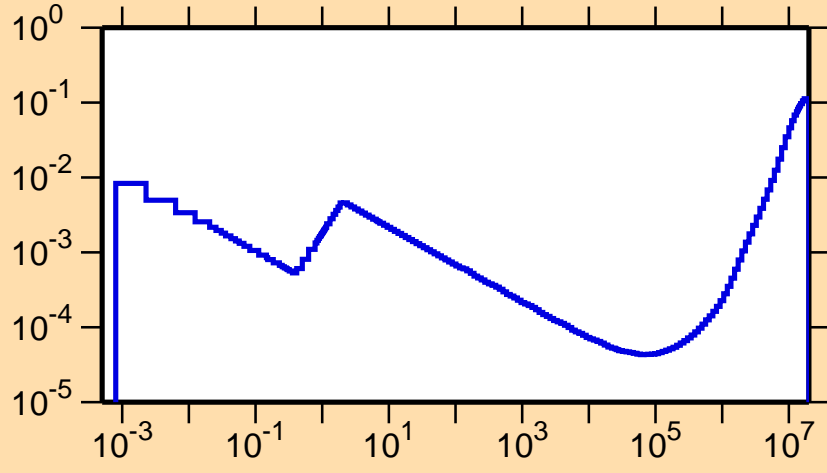
\sigma vs. E for ^{202}\text{Rn}(n,p)
