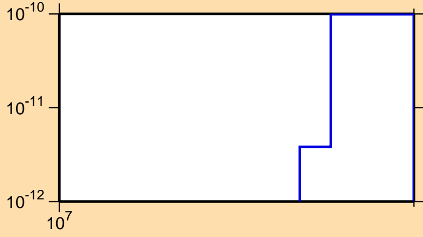
\sigma vs. E for ^{202}\text{Rn}(n,\text{pt})
