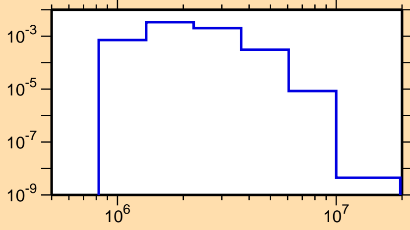
\sigma vs. E for ^{202}\text{Rn}(n,n_2)
