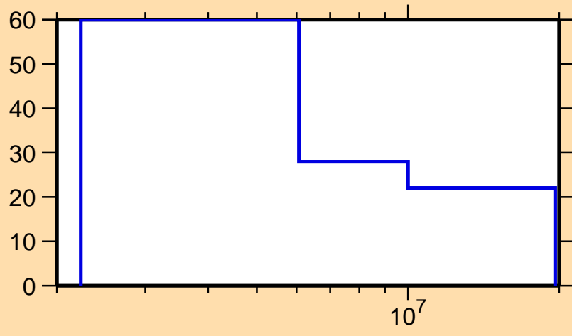
\Delta\sigma/\sigma vs. E for ^{202}\text{Rn}(n,n\text{cont.})
