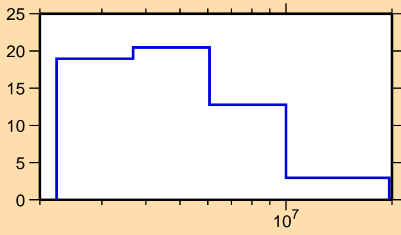
\Delta\sigma/\sigma vs. E for ^{202}\text{Rn}(n,\text{tot.})
