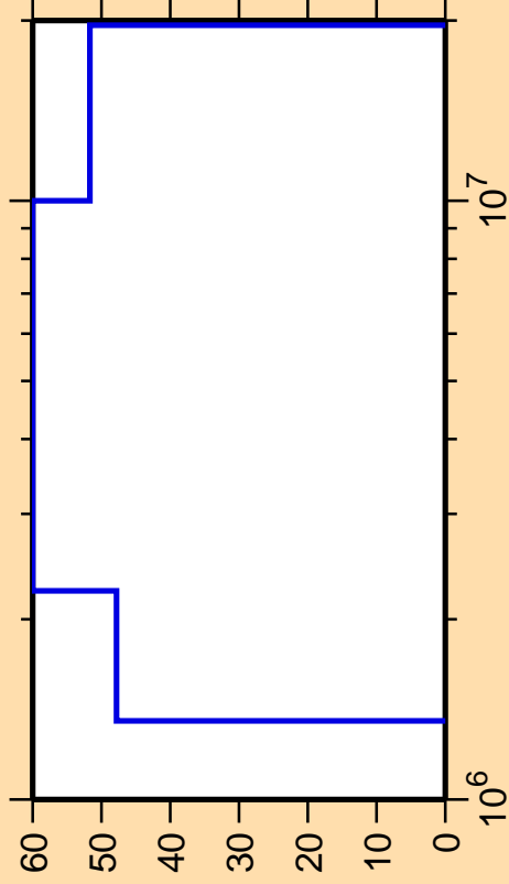
\Delta\sigma/\sigma vs. E for ^{202}\text{Rn}(n,n_4)
