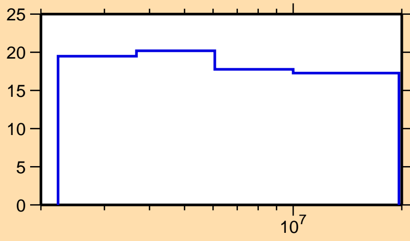
\Delta\sigma/\sigma vs. E for ^{202}\text{Rn}(n,n\text{onel.})
