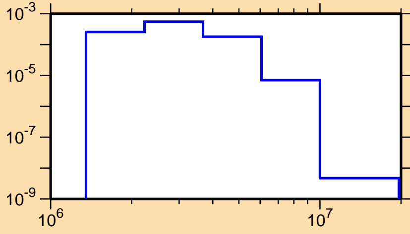
\sigma vs. E for ^{202}\text{Rn}(n,n_4)
