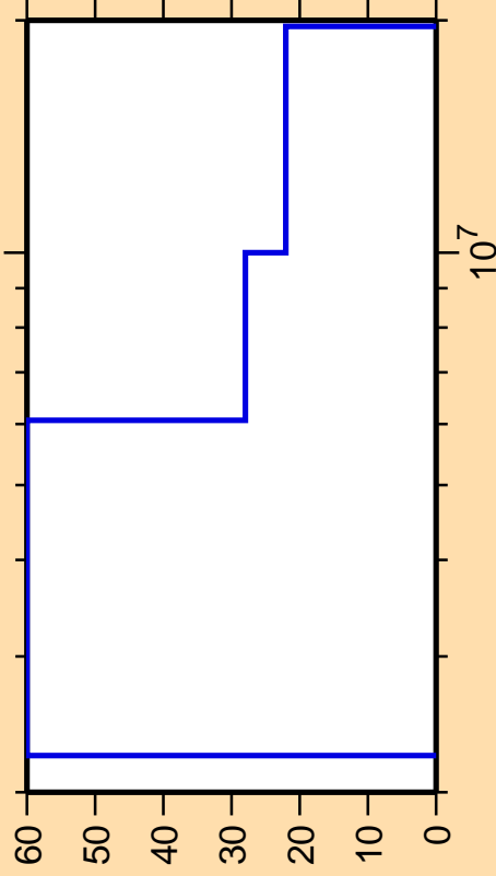
\Delta\sigma/\sigma vs. E for ^{202}\text{Rn}(n,n\text{cont.})
