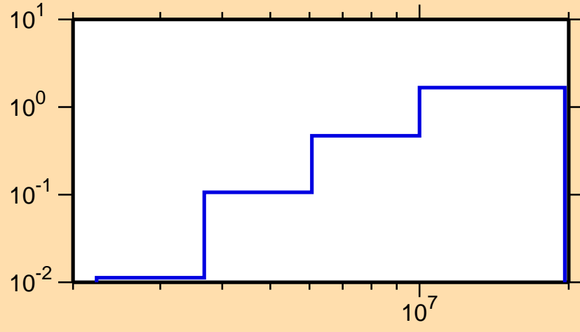
\sigma vs. E for ^{202}\text{Rn}(n,n\text{cont.})
