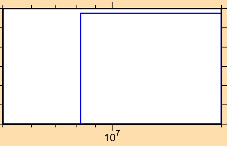
\sigma vs. E for ^{202}\text{Rn}(n,2np)
