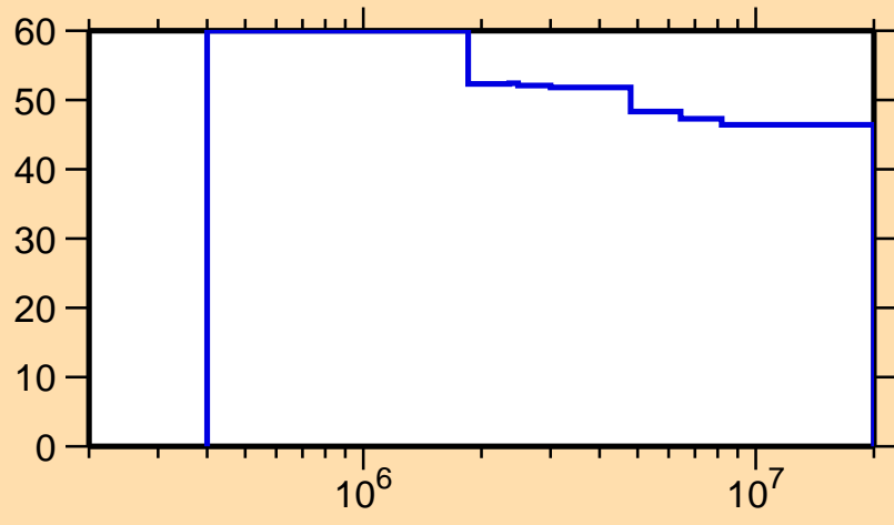
\Delta\sigma/\sigma vs. E for ^{202}\text{Rn}(n,n_1)
