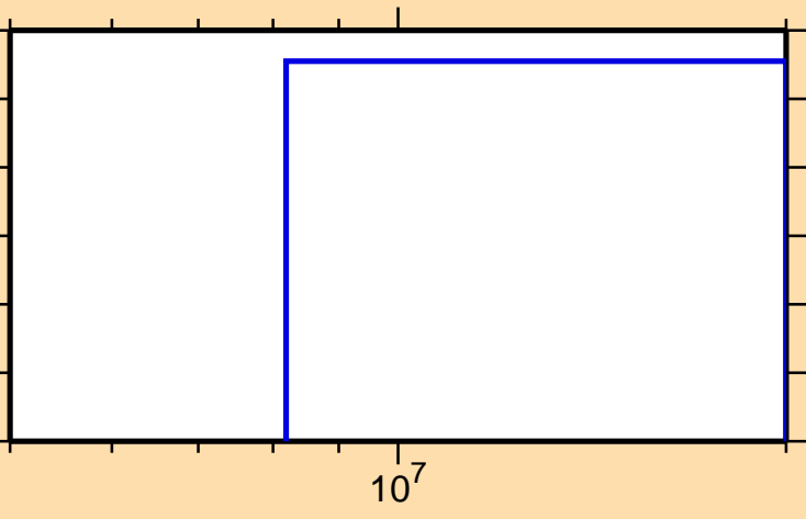
\sigma vs. E for ^{202}\text{Rn}(n,3n)
