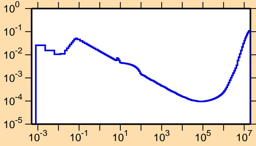
\sigma vs. E for ^{203}\text{Rn}(n,p)
