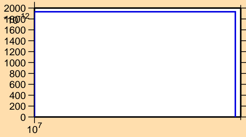
\sigma vs. E for ^{203}\text{Rn}(n,nd)
