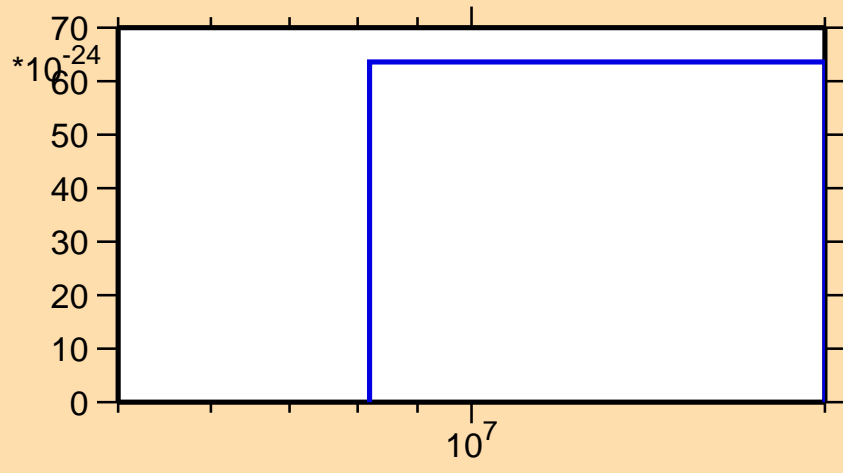
\sigma vs. E for ^{203}\text{Rn}(\text{mt } 11)
