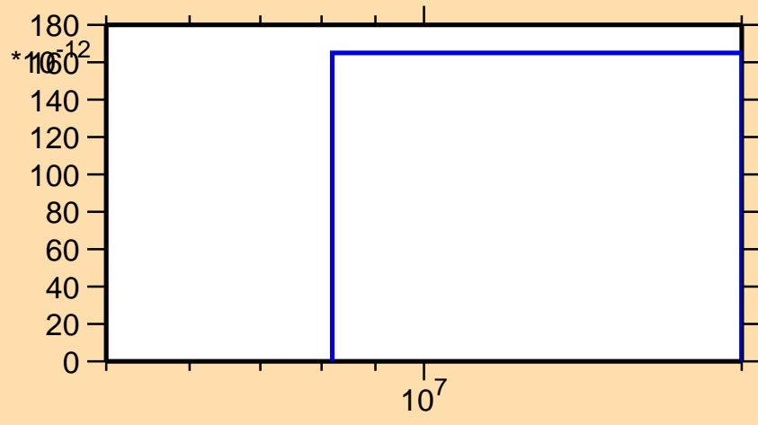
\sigma vs. E for ^{203}\text{Rn}(\text{mt } 45)
