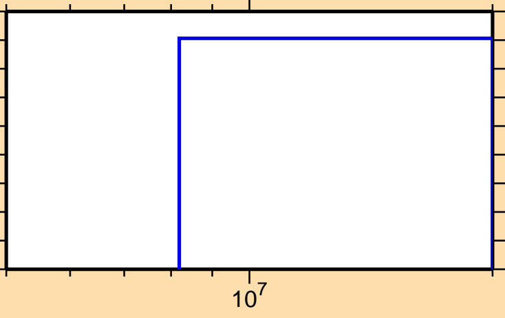
\sigma vs. E for ^{203}\text{Rn}(n,\text{nd})
