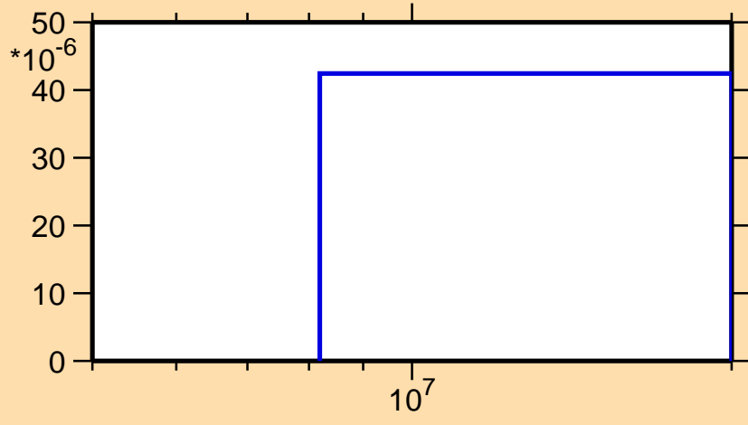
\sigma vs. E for ^{204}\text{Rn}(n,t)
