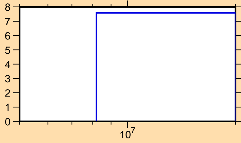
\Delta\sigma/\sigma vs. E for ^{204}\text{Rn}(n,\text{tot.})
