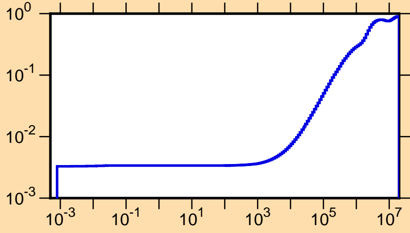
\mu vs. E for ^{205}\text{Rn}(\text{mt251})
